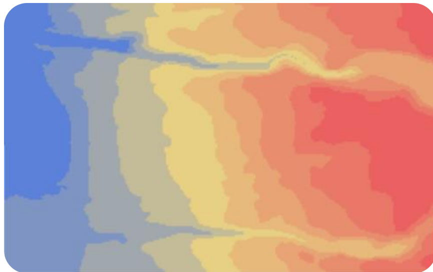
Sample "Relative Elevation" raster output
